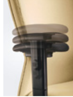
Arm height adjustment A push button allows arm height to be adjusted and locked into one of eight positions within a 3" range.
